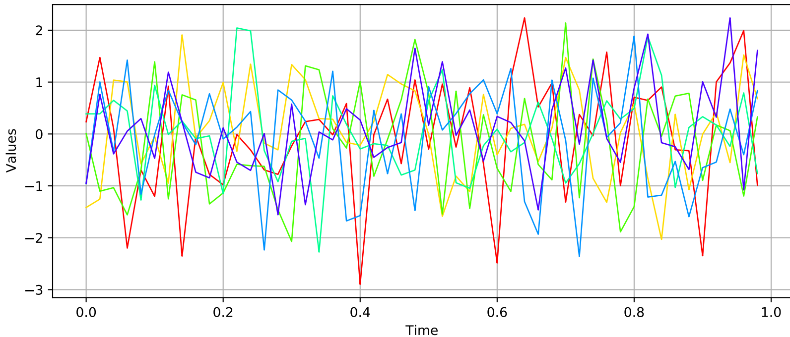
AggregatedProcess([WhiteNoise(Normal(mu = 0, sigma = 1))])
