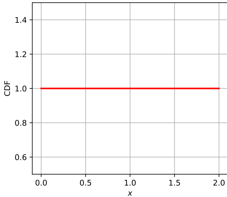
KPermutationsDistribution(k = 1, n = 1)
