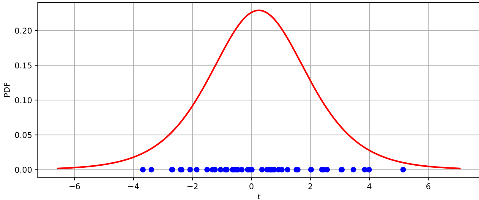
Logistic( \mu = 0.250138 , \beta = 1.09154 )
