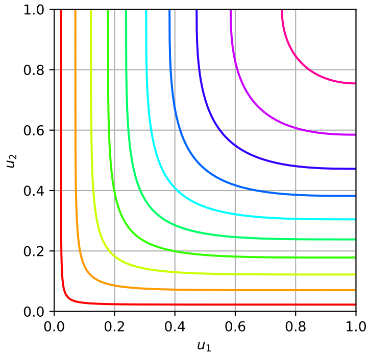
NormalCopula(R = [[ 1 0.8 ]]
