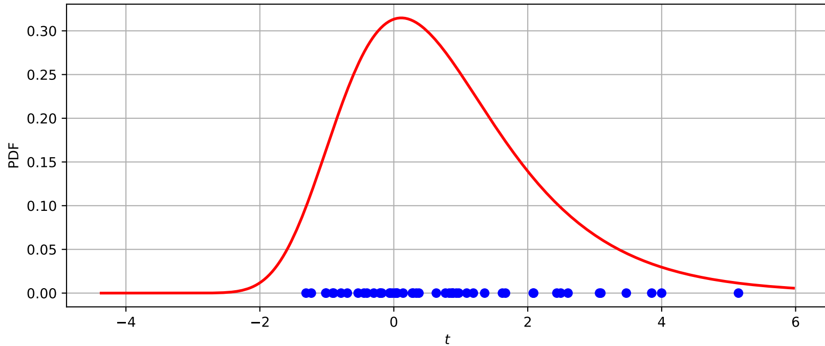
Gumbel(beta = 1.16859, gamma = 0.111393)
