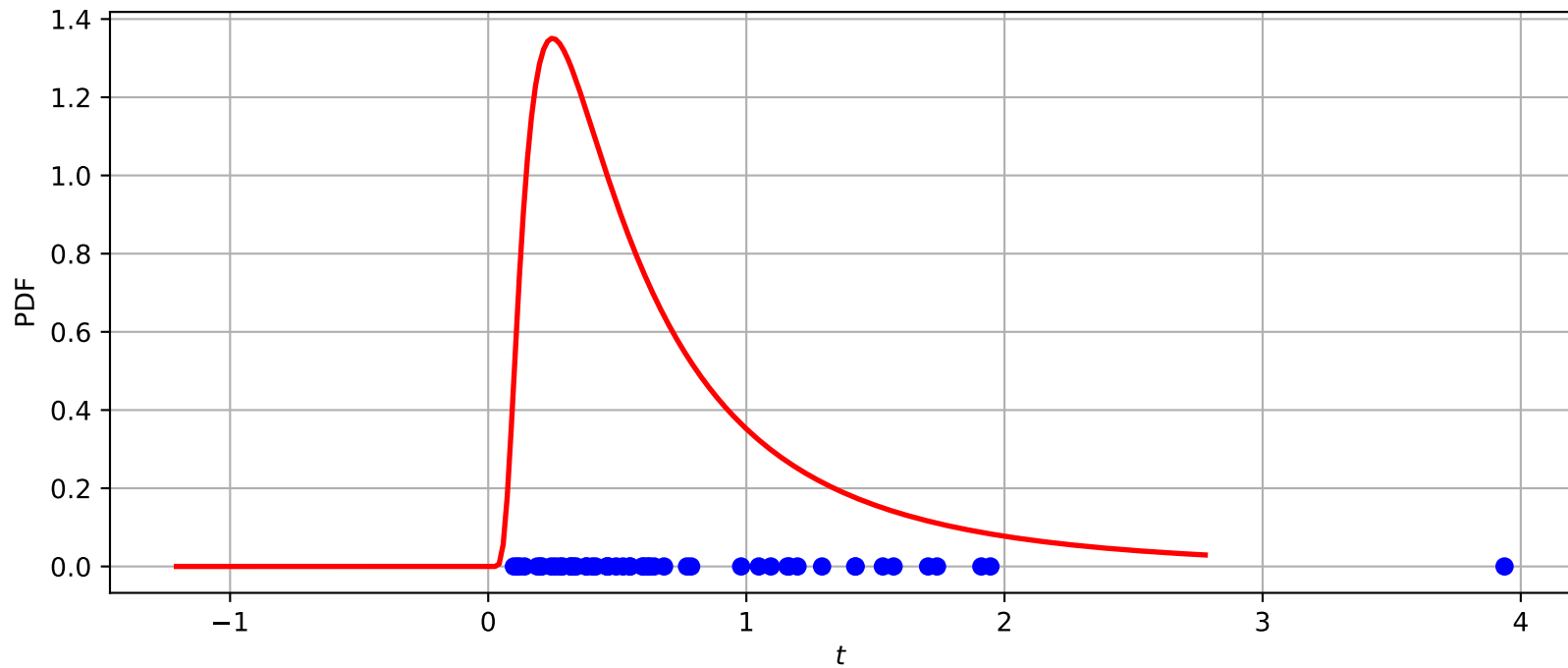
InverseNormal( \mu = 0.779711 , \lambda = 0.831379 )
