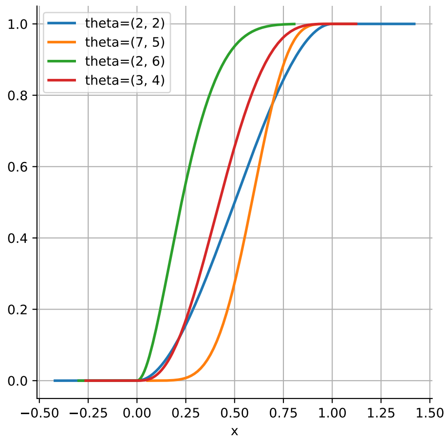
CDFs of 1D Dirichlet distributions
