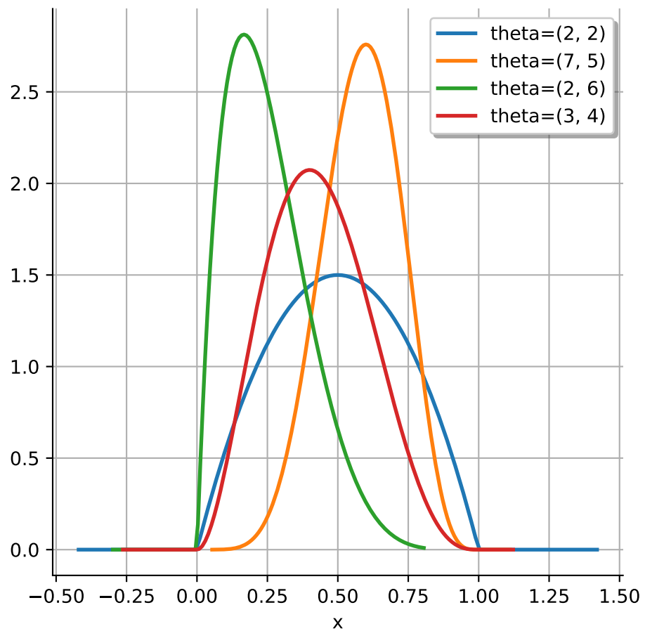
PDFs of 1D Dirichlet distributions
