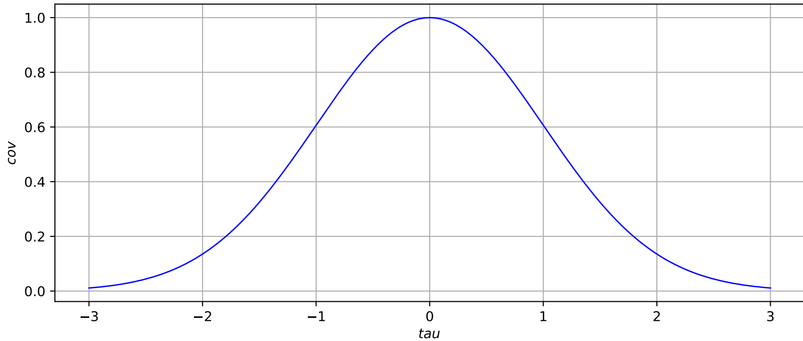
SquaredExponential(scale=[1], amplitude=[1])
