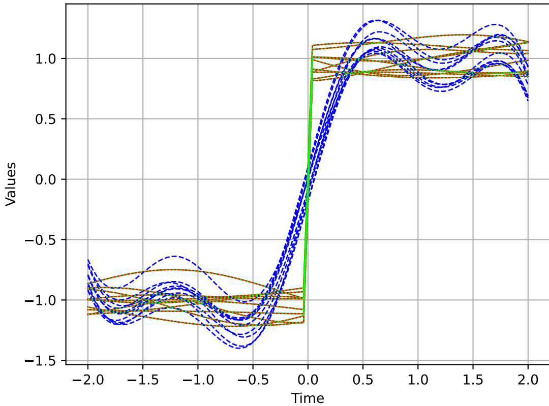
reduction of sign(x) w/o trend - 0 marginal
