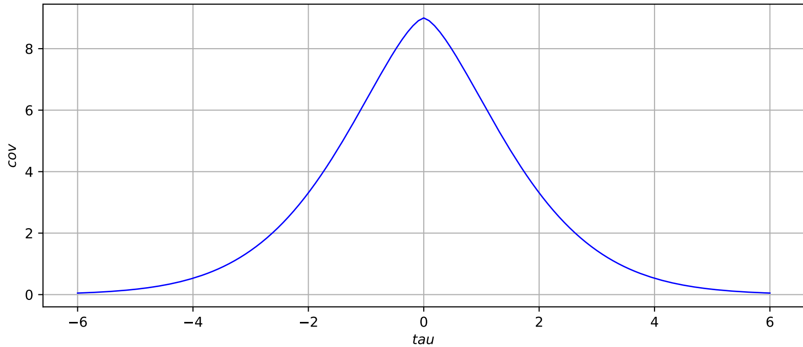
GeneralizedExponential(scale=[2], amplitude=[3], p=1.5)
