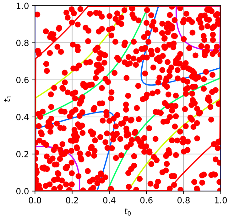
PlackettCopula(theta = 2.40566)
