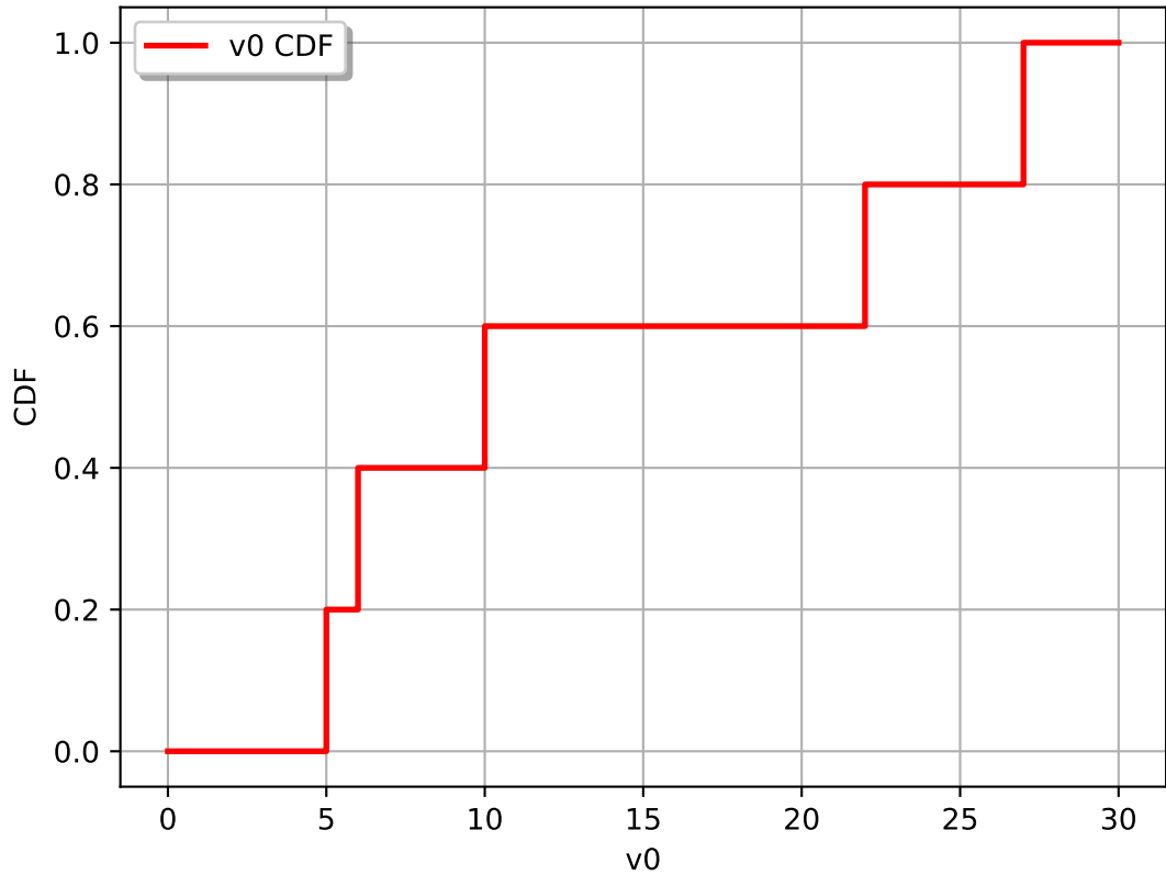
Empirical CDF
