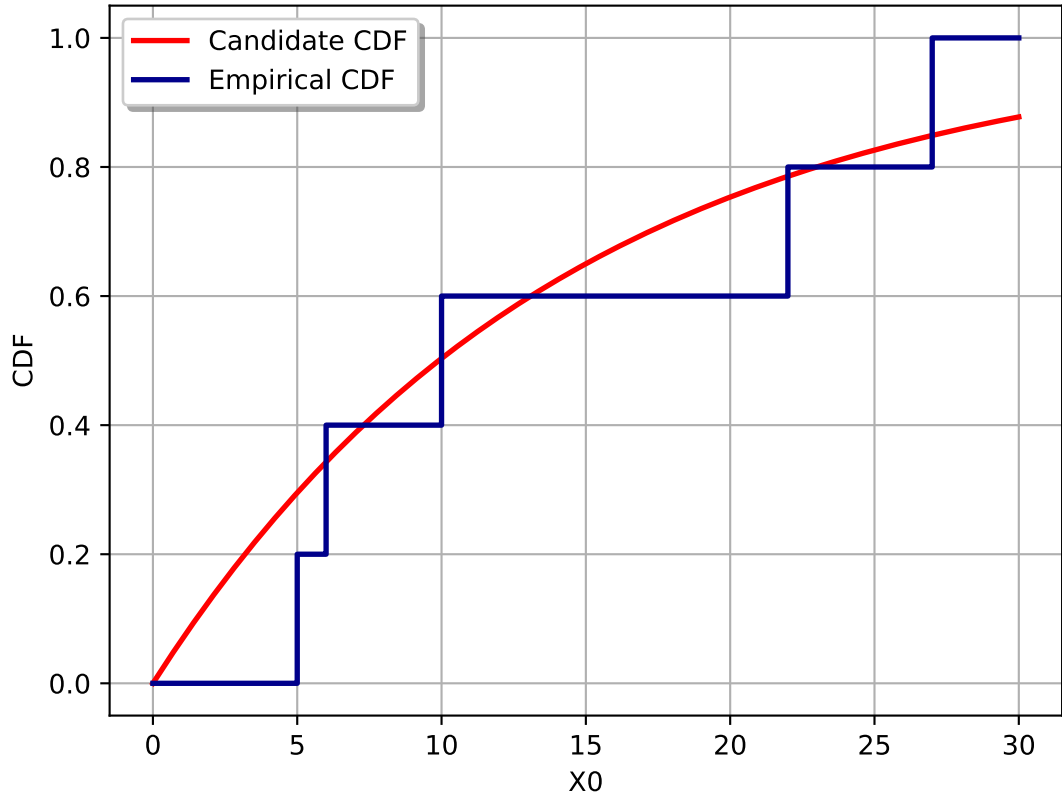
CDF comparison
