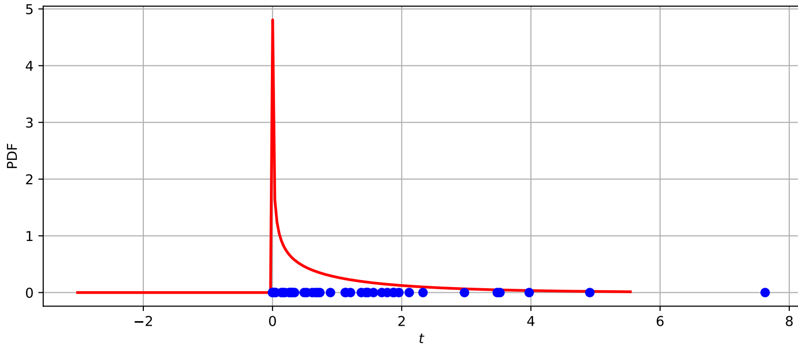
ChiSquare(nu = 1.20302)
