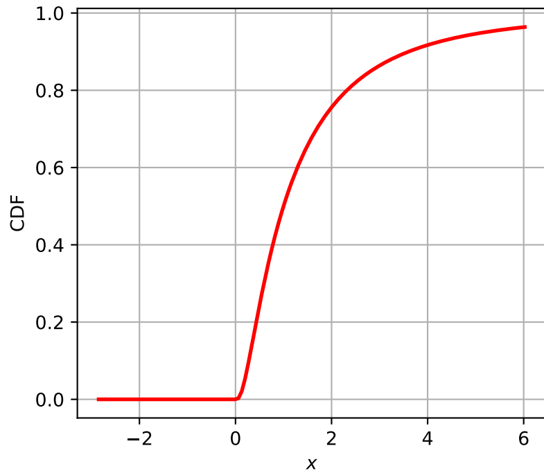
LogNormal( \mu_{\text{Log}} = 0 , \sigma_{\text{Log}} = 1 , \gamma = 0 )
